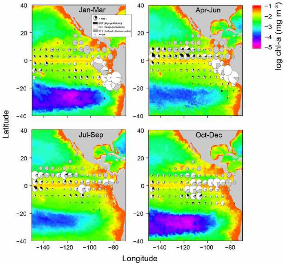
FIGURE L-11. Mean log chlorophyll-a concentration (in \text{mg m}^3 ) for each quarter during 2021 with catches of tropical tunas overlaid. Chlorophyll data obtained from NOAA CoastWatch on January 20, 2022, “Chlorophyll, NOAA, VIIRS, Science Quality, Global, Level 3, 2012-present, Monthly”, NOAA NMFS SWFSC ERD, https://coastwatch.pfeg.noaa.gov/erddap/info/nedisVHNSQchlaMonthly/index.html .
